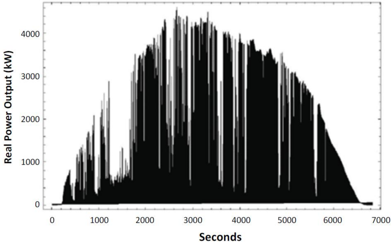
Solar Energy at 10 Second Resolution
