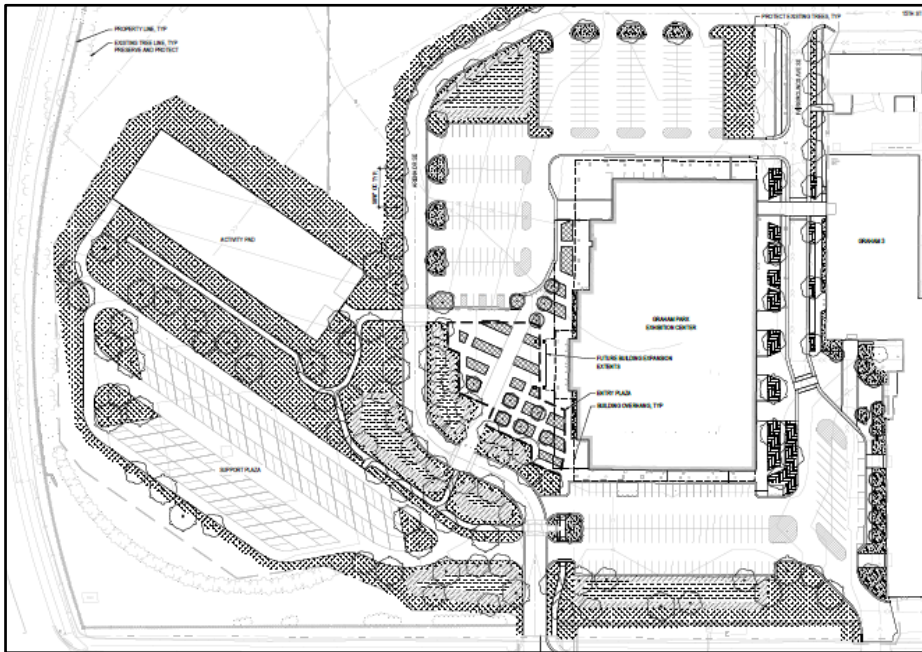
Graham Park Regional Exhibition Center and outdoor improvements site plan.
