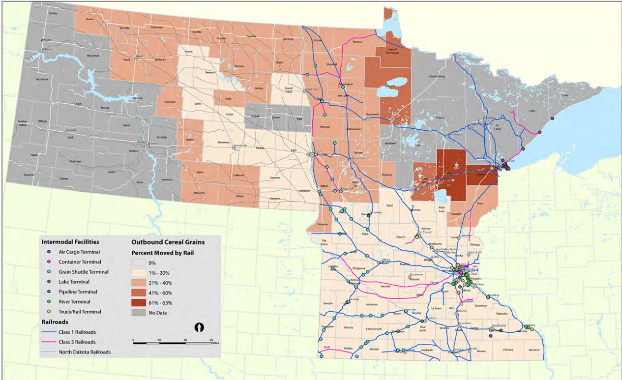
Outbound Cereal Grains (Corn, Soy, Wheat) Rail Share
