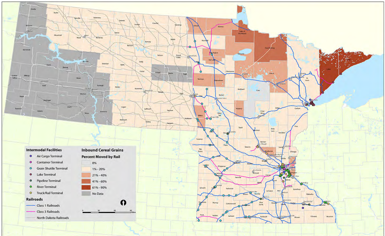
Inbound Cereal Grains (Corn, Soy, Wheat) Rail Share
