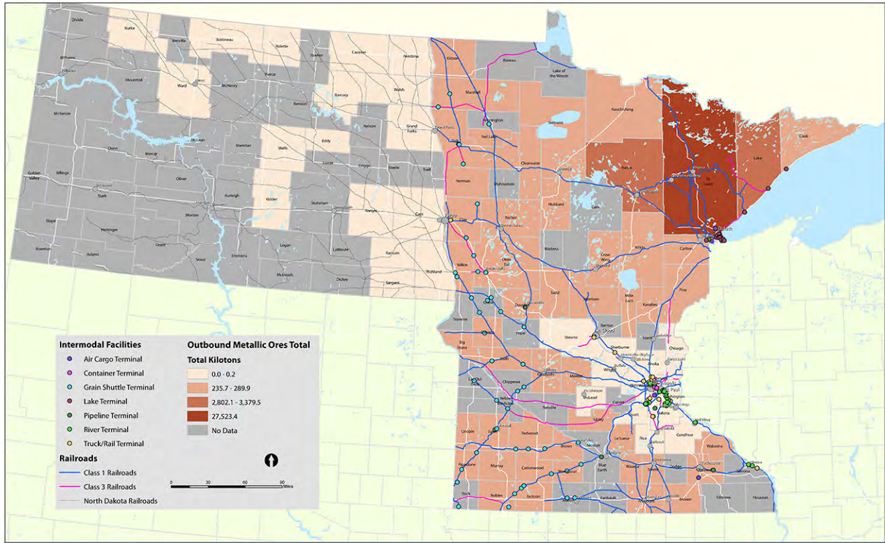
Outbound Metallic Ores Tonnage
