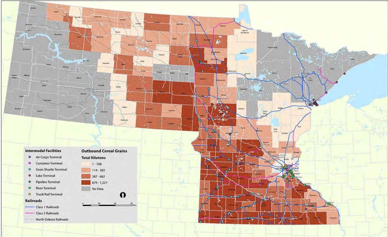
Outbound Cereal Grains (Corn, Soy, Wheat) Tonnage
