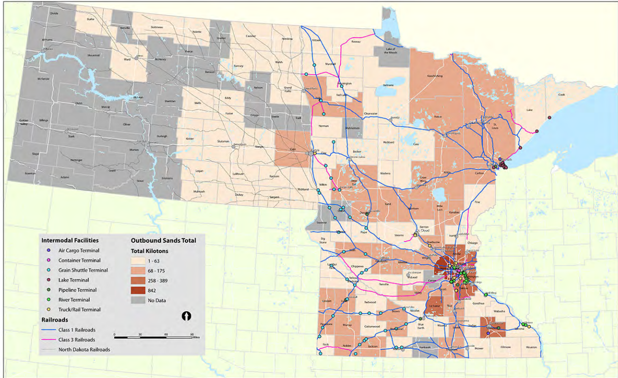
Outbound Natural Sands Tonnage
