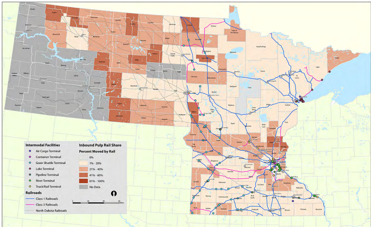
Inbound Pulp, Newsprint, Paper, & Paperboard Rail Share
