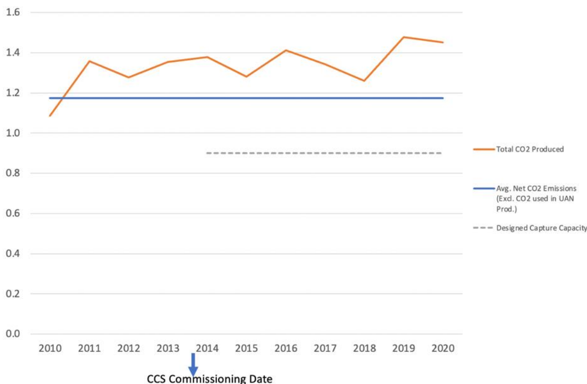
Figure 23: Coffeyville CCS CO 2 Emissions vs Maximum Capturing Capacity (2010–2020)
