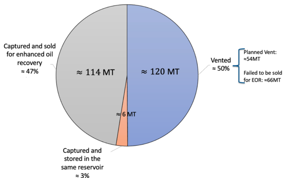
Figure 7: Shute Creek CCUS Lifetime CO 2 Capture Performance
